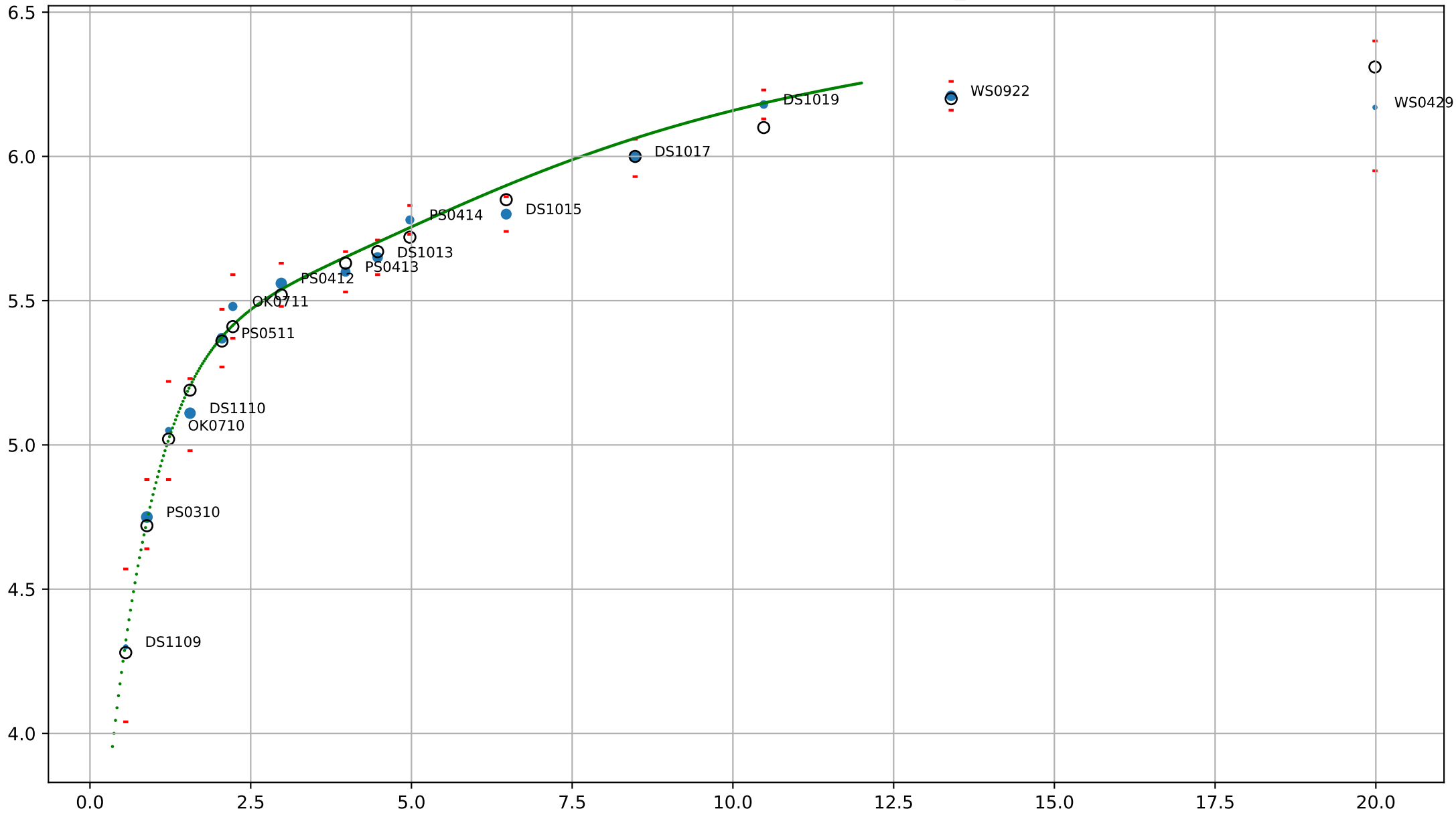
Yield curve as of 2009-04-30 00:00:00 ObFuVal: 0.8848, Diff_avg: 0.0447 pct points
