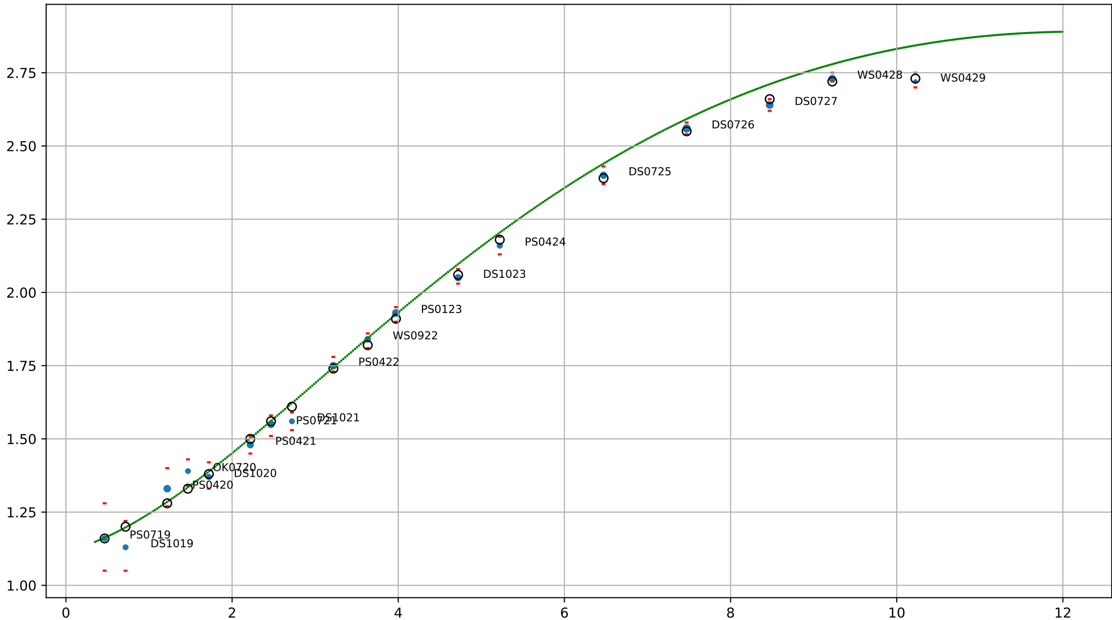
Yield curve as of 2019-02-01 00:00:00 ObFuVal: 0.1547, Diff_avg: 0.0228 pct points
